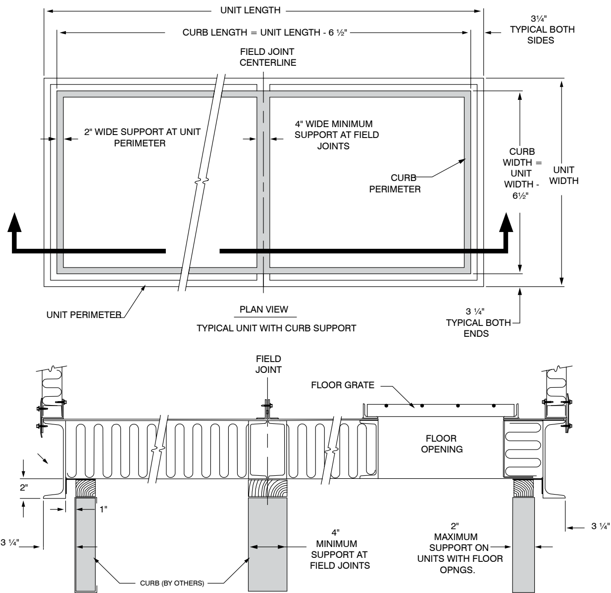
SECTION SELF FLASHING UNIT BASE SHOWING CURB SUPPORT REQUIREMENTS
