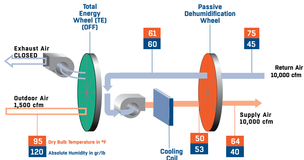
FIGURE 4 Schematic of the Pinnacle system operating in unoccupied mode. The system can operate in 100% recirculation mode and with very little refrigeration input effectively controlling the indoor humidity.
