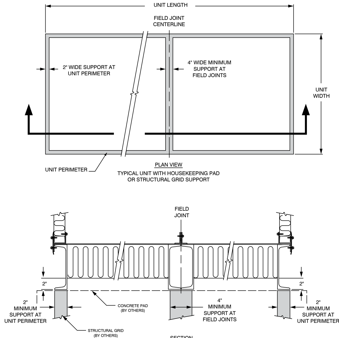
SECTION UNIT BASE WHEN MOUNTING ON PAD OR STRUCTURAL GRID
