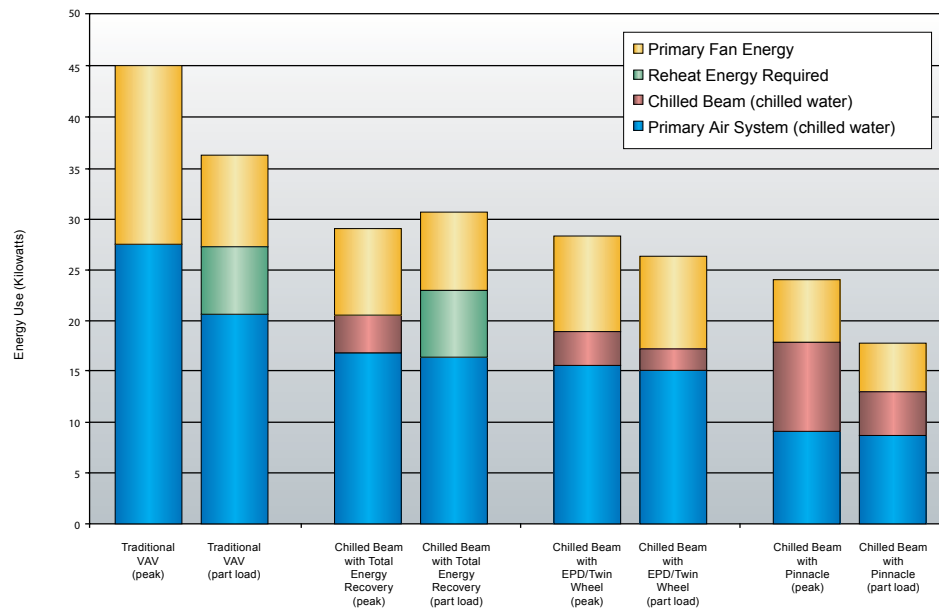
Figure 12: Modeled results comparing energy consumed by the VAV and chilled beam approaches
