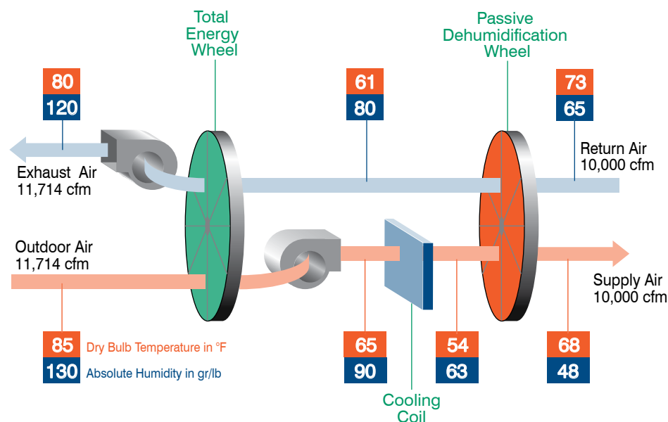
Figure 4: Typical Pinnacle cooling season performance
