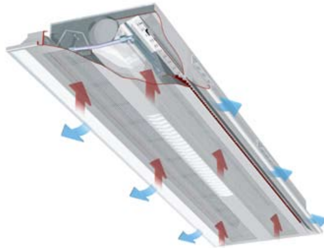
Figure 1: Graphic of FläktGroup SEMCO's Flexicool® Chilled Beam
