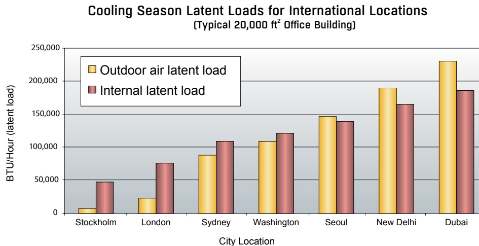
Figure 3: Indoor and outdoor latent loads for a 20,000 ft 2 office in various cities globally
