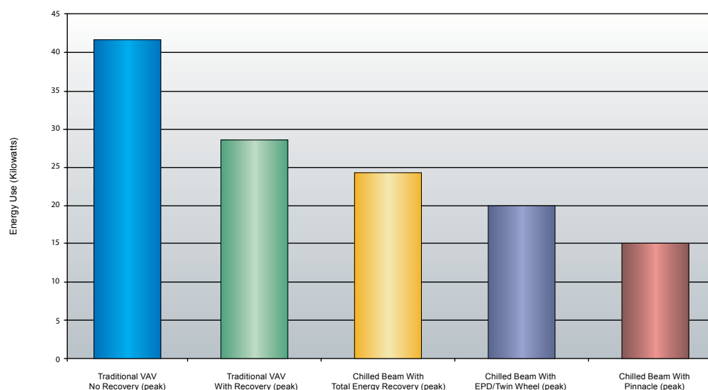
Figure 11: Primary air-cooling capacity required with VAV shown with and without total recovery
