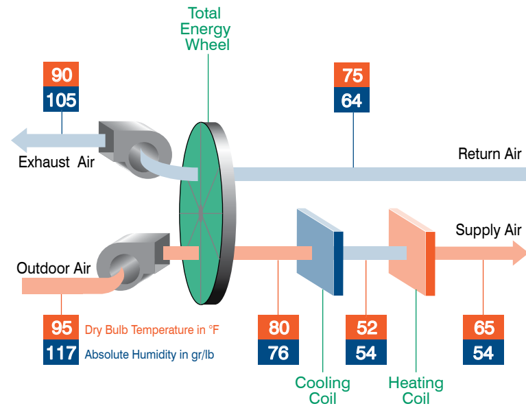
Figure 7: Single total energy wheel with reheat
