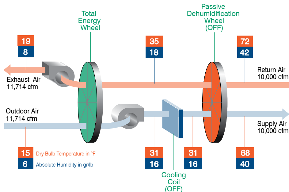
Figure 6: Pinnacle system in the heating mode
