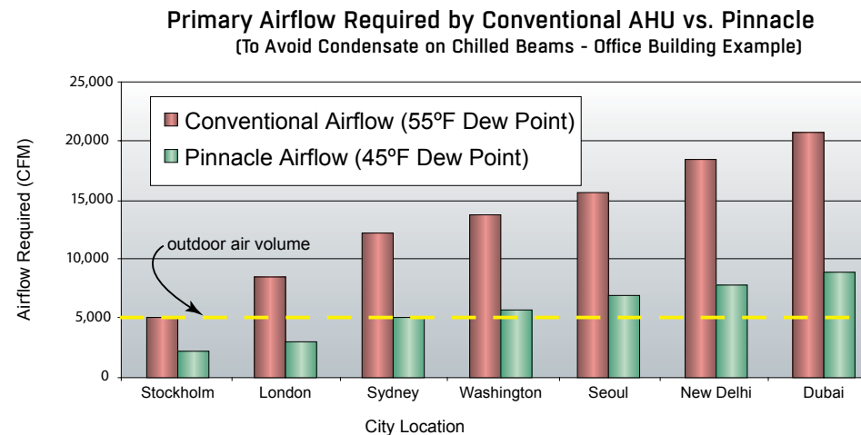
Figure 10: Comparing primary airflow required by conventional and Pinnacle systems
