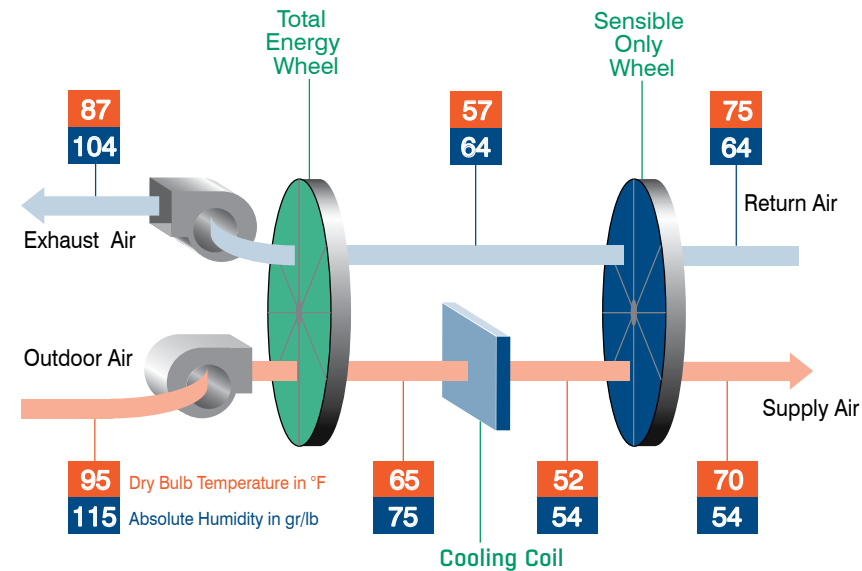
Figure 8: FläktGroup SEMCO EPD dual total energy wheel with free reheat
