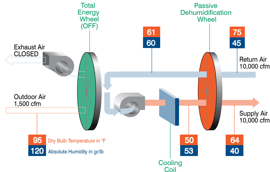
Figure 5: Pinnacle system in the unoccupied mode
