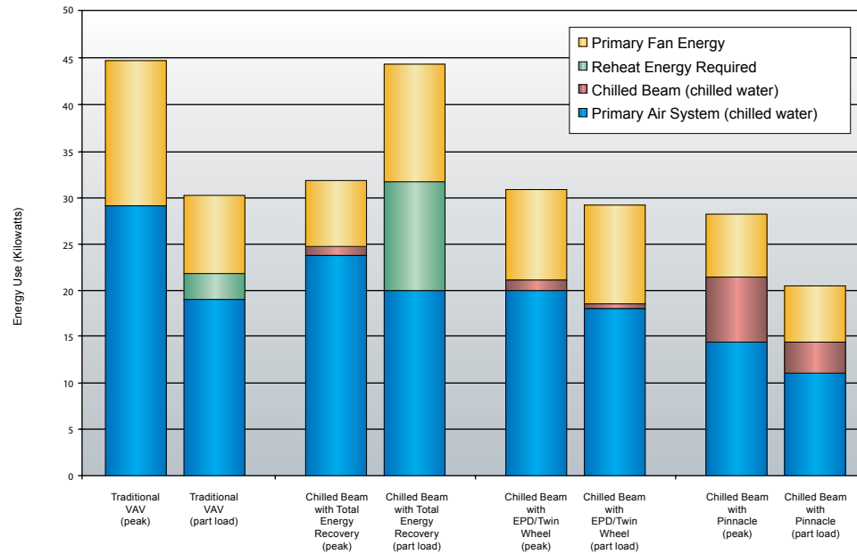
Figure 14: Modeled results comparing energy consumed by the VAV and chilled beam approaches
